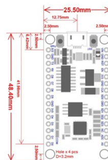
Figure .4: NodeMCU 2D View ESP8266 NODE MCU
