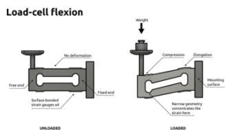
Figure .8 : Load-cell Flexion
