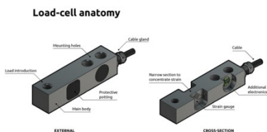
Figure .7: Load-cell Anatomy
