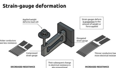
Figure .9: strain-Gauge Deformation
